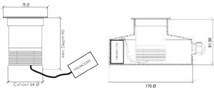
Concrete Housing
