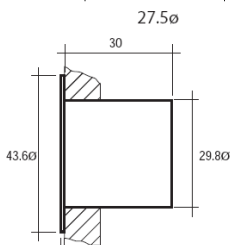
Stainless steel installation sleeve with flange
