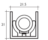
'U' channel for 12.8Ø Light Tube
