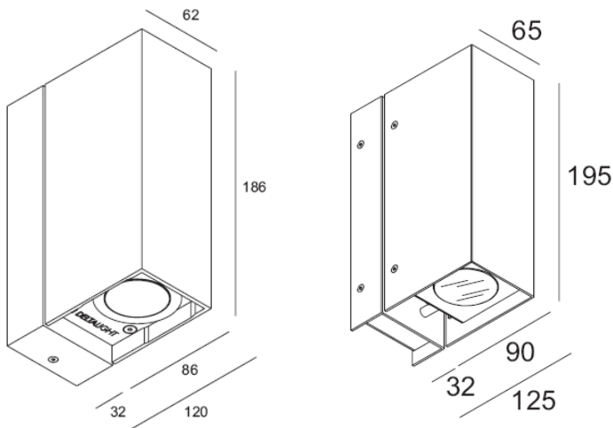
Inox Version
