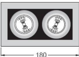
Shomei 2 Cut out: 80 x 160mm
