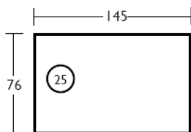
Mounting canister
